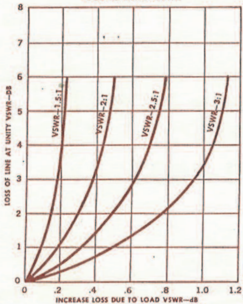
ADDITIONAL ATTENUATION DUE TO LOAD VSWR
