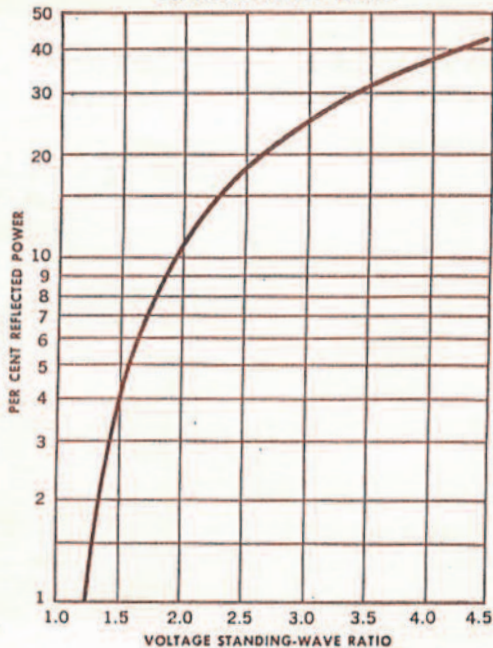
REFLECTED POWER vs STANDING-WAVE RATIO
