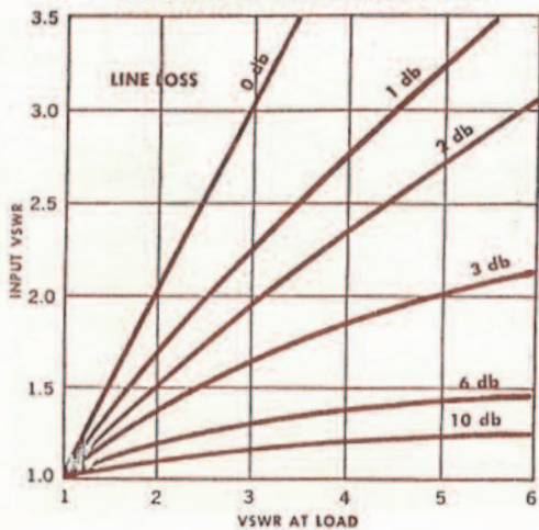
REDUCTION OF VSWR AS A RESULT OF LINE ATTENUATION
